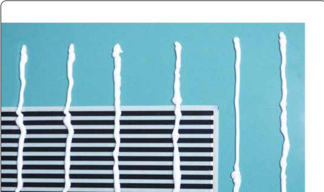
Apply mirror adhesive to the back of the mirror in vertical beads.
