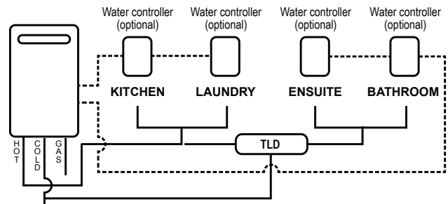
Diagram 2 : NOT a 50°C Appliance
