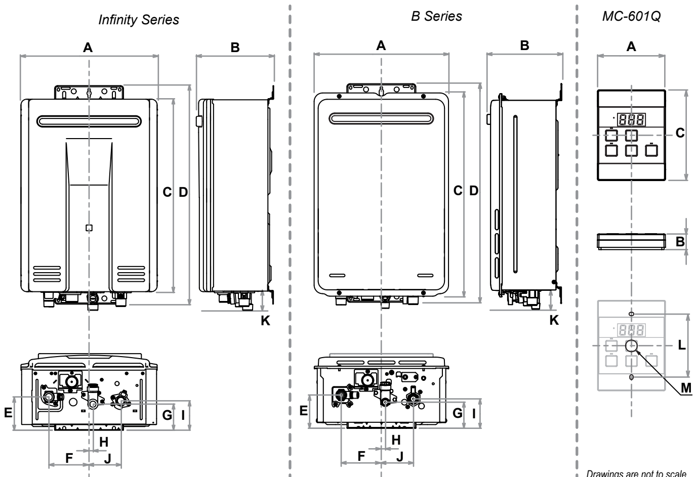
DIAGRAM 1. DIMENSIONS
