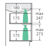
SIDE VIEW: RECESS & DRAWER STORAGE
